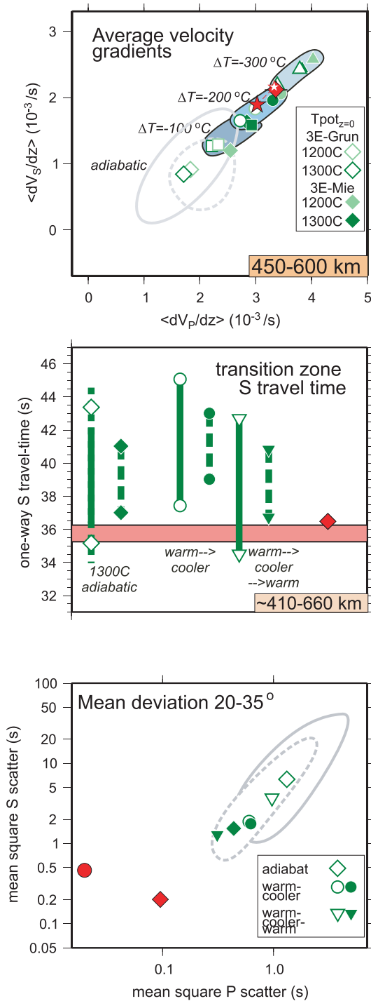
Figure 7. Alternative, non-adiabatic thermal structures tested against seismic data. Introducing a drop in adiabat temperature of ~200°C in the lower transition zone (irrespective of the absolute temperature) improves the fit to the velocity gradients, but a return to warmer temperatures is required to fit the SS-precursors, and does not significantly improve the fit to direct travel times. Refer to Figs 2 and 3 for further explanation of symbols.
