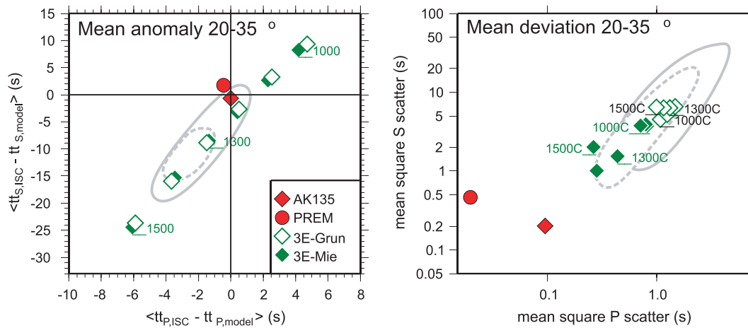
Figure 6. Direct P - and S -travel time misfits for adiabatic pyrolites at a range of potential temperatures (1000–1500°C). Refer to Figs 2 and 3 for further explanation of symbols. The mean square misfit (right-hand panel) is not reduced by uniform shifts in adiabatic temperature.
