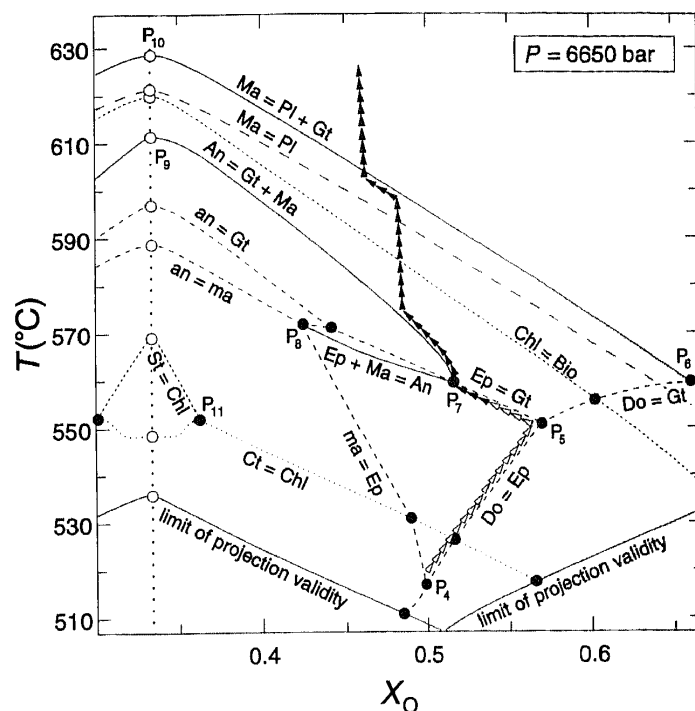
Fig. 7. Isobaric ( P = 6650 bars) T - X_0 phase diagram section for the system shown in Fig. 5, with the additional constraint that all phase relations are stable with phengitic muscovite. Curves are labeled by reactions with high-temperature assemblages to the right of equals signs. Maximum \text{H}_2\text{O} activity occurs at X_0 = 1/3 (vertical dotted line) in \text{C-O-H} fluids (Connolly and Cesare, 1993). Solid curves represent nondegenerate equilibria; dashed curves represent Na-free equilibria; short-dashed curves represent AFM phase relations. Solid arrows indicate T - X_0 evolution of inclusions and matrix calc-silicates, as inferred from textural relationships. Open arrows illustrate a T - X_0 path given that the high- X_0 fluid composition originated from the decarbonation of dolomite. Mineral compositions at selected invariant (solid circles) and singular (open circles) points are given in Table 3; notation is as in Table 1. See Appendix 1 for computational details.
