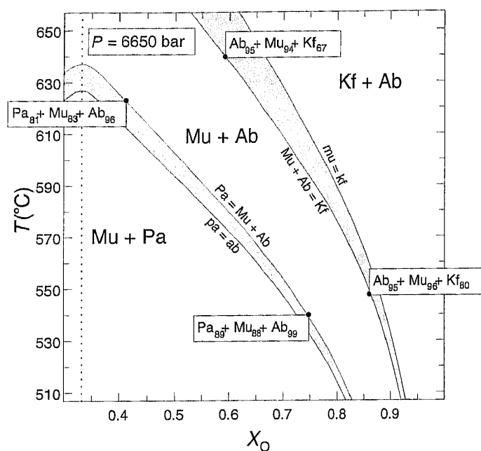
Fig. 9. Isobaric ( P = 6650 bars) T - X_O phase diagram section for the quartz + kyanite + graphite-saturated system \text{Na}_2\text{O} - \text{K}_2\text{O} - \text{Al}_2\text{O}_3 - \text{SiO}_2 - \text{C} - \text{O} - \text{H} . Substantially more O-rich fluid compositions than those inferred for calc-silicate microinclusions (point P_7 ; Fig. 8) are required to explain albite + muscovite and orthoclase + albite associations observed in early garnet. The vertical dotted line locates the X_O = 1/3 fluid composition. Mineral compositions at selected invariant (solid circles) points are given in Table 3; notation is as in Table 1. See Appendix 1 for computational details.
