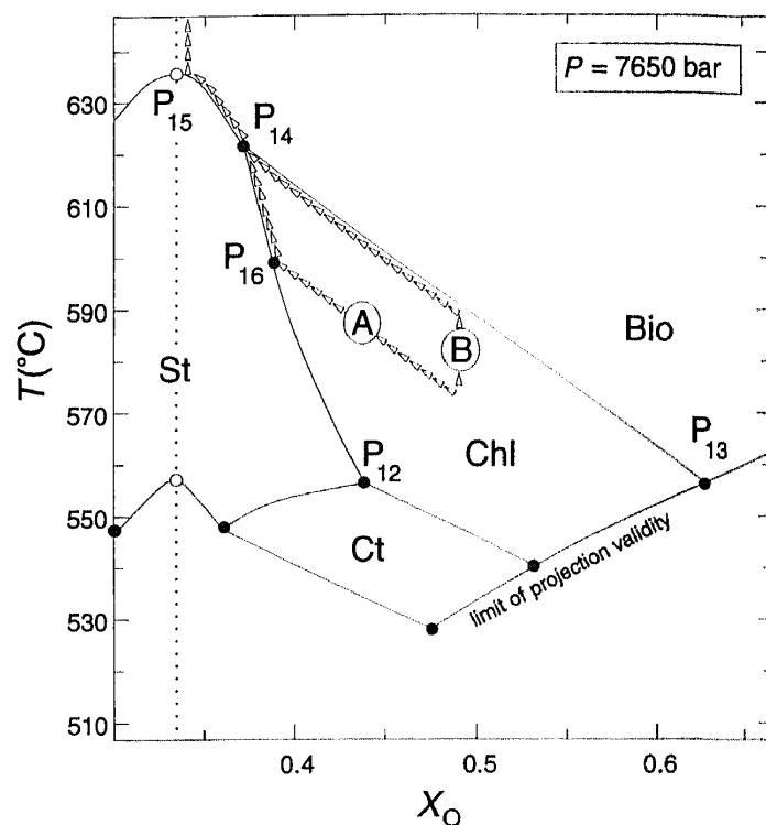
Fig. 10. Isobaric ( P = 7650 bars) T - X_O phase diagram section showing stable AFM phases in the rutile + quartz + kyanite + graphite + ilmenite-saturated system \text{MgO} - \text{FeO} - \text{K}_2\text{O} - \text{Al}_2\text{O}_3 - \text{SiO}_2 - \text{TiO}_2 - \text{C} - \text{O} - \text{H} . The vertical dotted line locates the X_O = 1/3 fluid composition. Arrows indicate possible T - X_O evolution paths for the fluid phase.
