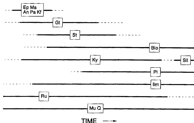
Fig. 4. Paragenetic sequence of the metapelite minerals as deduced from textural relationships. Coeval minerals, in particular microinclusions, were not necessarily in mutual equilibrium.
