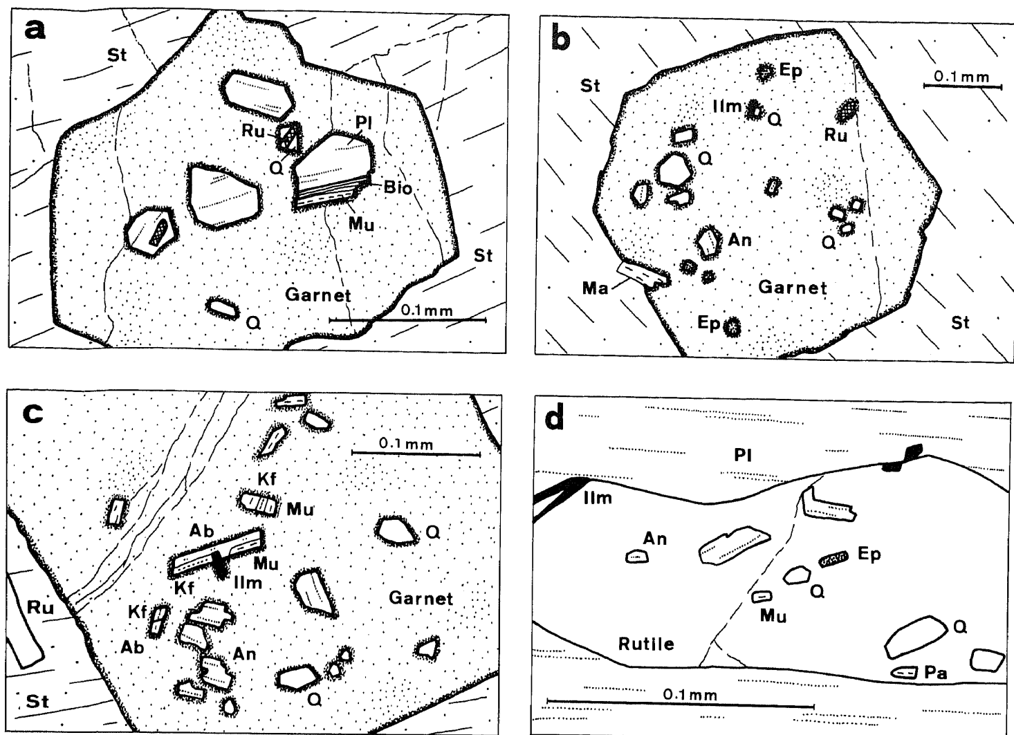
Fig. 3. Sketches from SEM photographs of microinclusions in garnet and rutile (see Table 1 for notation): (a) cloudy garnet (core \text{Gr}_{90}\text{Py}_{10}\text{Al}_{74}\text{Sp}_7 , rim \text{Gr}_{60}\text{Py}_{40}\text{Al}_{74}\text{Sp}_{11} ) with inclusions of plagioclase ( \text{An}_{42}\text{--}\text{An}_{49} ), muscovite ( \text{Mu}_{83,4,7} ), biotite ( \text{Bio}_{57,28,13} ), quartz, and rutile; (b) clear garnet (core \text{Gr}_{27}\text{Py}_{6}\text{Al}_{62}\text{Sp}_5 , rim \text{Gr}_{16}\text{Py}_{10}\text{Al}_{66}\text{Sp}_8 ) with inclusions of anorthite ( \text{An}_{91}\text{--}\text{An}_{97} ), epi-
