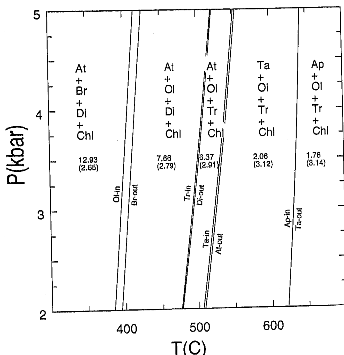
Fig. 3 Predicted phase relations for the Malenco serpentinite (lherzolite) bulk composition as a function of pressure and temperature as discussed in the text and table 2. In each field the approximate water content (wt%) and, in parentheses, density ( \text{g/cm}^3 ) are given. Because of solution behaviour none of the phase fields are bounded by univariant reactions, rather each 4-phase field is bound by a narrow 5-phase field in which the modal mineralogy varies rapidly. These 5-phase fields correspond to the isograds observed in the Malenco serpentinite.
